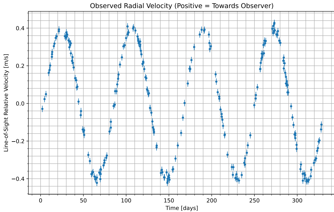
Figure 1: We have isolated the radial velocity of the host star due to the candidate planet. Data begins at UTC 2076-04-12/16:34. Positive values indicate the velocity at which the star is moving towards us; negative indicate the velocity at which it is moving away.
