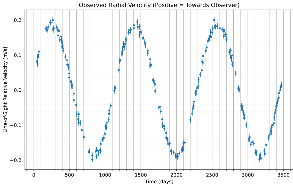
Figure 1: We have isolated the radial velocity of the host star due to the candidate planet. Data begins at UTC 2064-02-01/15:20. Positive values indicate the velocity at which the star is moving towards us; negative indicate the velocity at which it is moving away.
