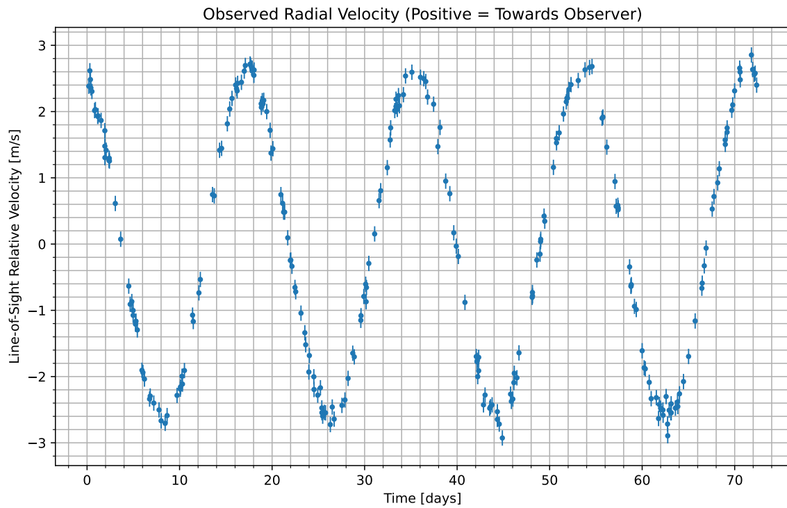
Figure 1: We have isolated the radial velocity of the host star due to the candidate planet. Data begins at UTC 2081-06-07/16:45. Positive values indicate the velocity at which the star is moving towards us; negative indicate the velocity at which it is moving away.
