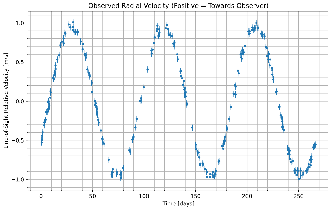
Figure 1: We have isolated the radial velocity of the host star due to the candidate planet. Data begins at UTC 2094-02-16/05:53. Positive values indicate the velocity at which the star is moving towards us; negative indicate the velocity at which it is moving away.
