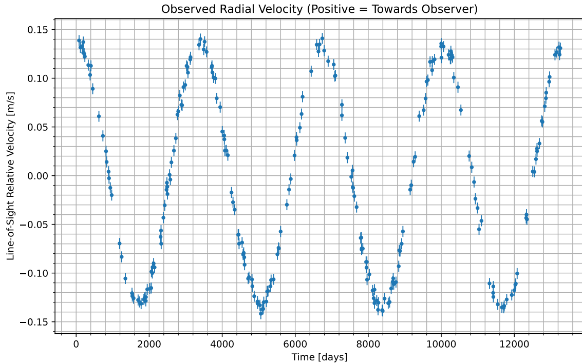
Figure 1: We have isolated the radial velocity of the host star due to the candidate planet. Data begins at UTC 2038-05-01/12:59. Positive values indicate the velocity at which the star is moving towards us; negative indicate the velocity at which it is moving away.
