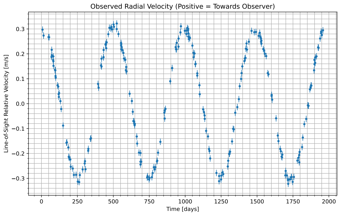
Figure 1: We have isolated the radial velocity of the host star due to the candidate planet. Data begins at UTC 2093-06-30/03:37. Positive values indicate the velocity at which the star is moving towards us; negative indicate the velocity at which it is moving away.
