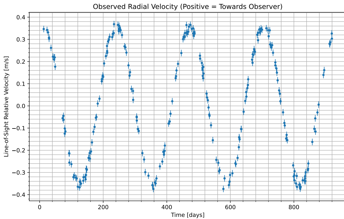
Figure 1: We have isolated the radial velocity of the host star due to the candidate planet. Data begins at UTC 2086-04-29/12:16. Positive values indicate the velocity at which the star is moving towards us; negative indicate the velocity at which it is moving away.
