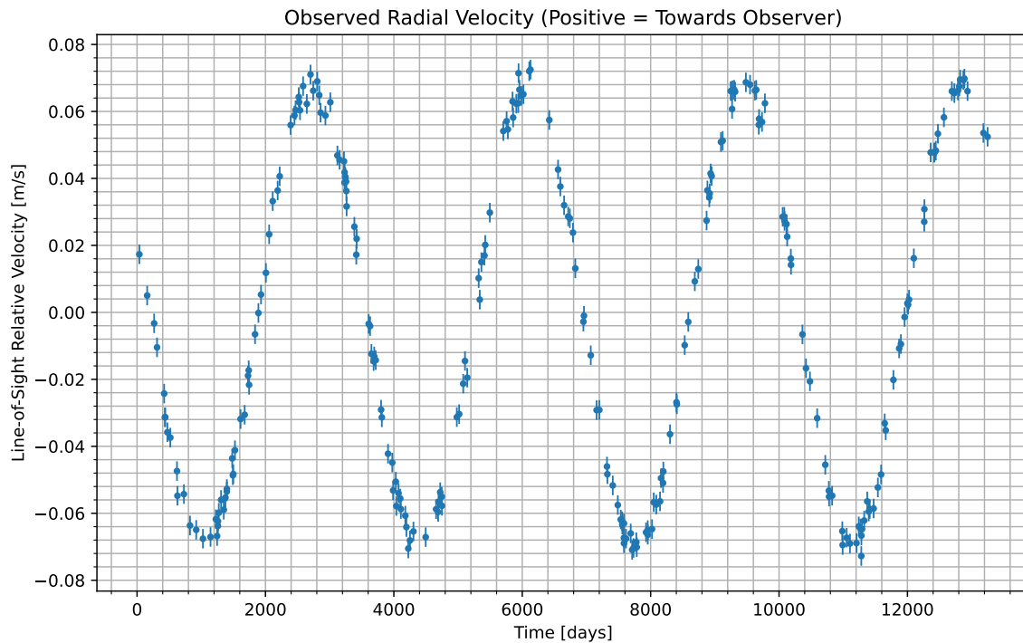
Figure 1: We have isolated the radial velocity of the host star due to the candidate planet. Data begins at UTC 2059-11-06/12:45. Positive values indicate the velocity at which the star is moving towards us; negative indicate the velocity at which it is moving away.
