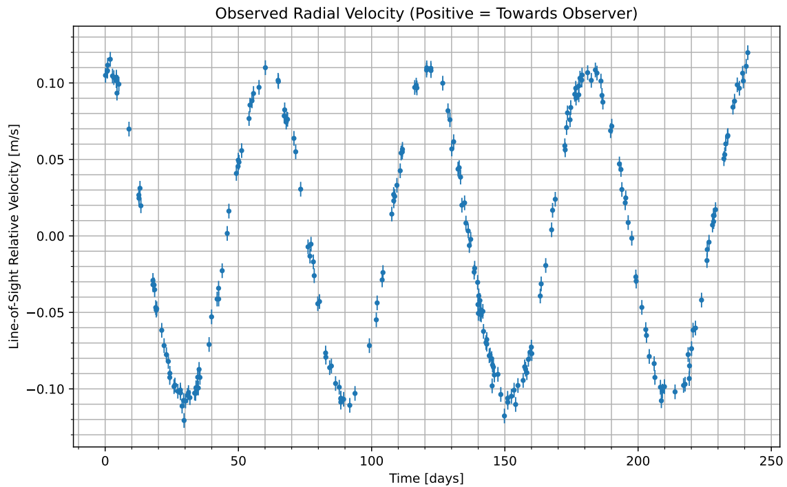
Figure 1: We have isolated the radial velocity of the host star due to the candidate planet. Data begins at UTC 2094-04-22/18:22. Positive values indicate the velocity at which the star is moving towards us; negative indicate the velocity at which it is moving away.
