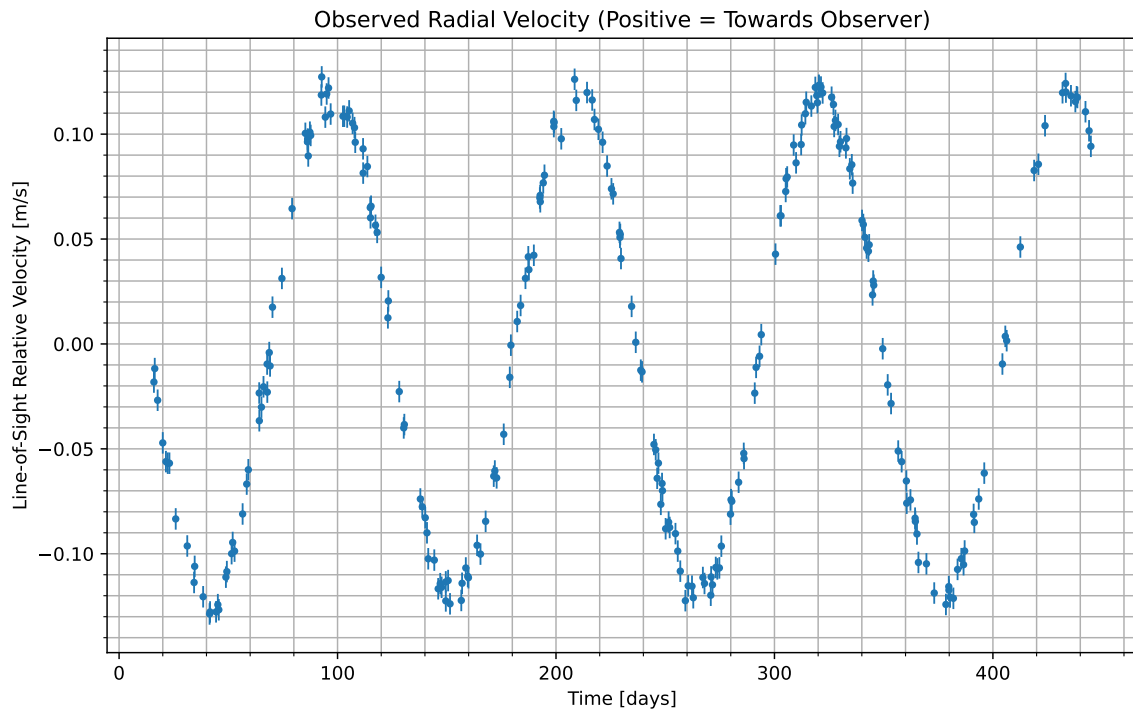
Figure 1: We have isolated the radial velocity of the host star due to the candidate planet. Data begins at UTC 2098-04-21/16:17. Positive values indicate the velocity at which the star is moving towards us; negative indicate the velocity at which it is moving away.
