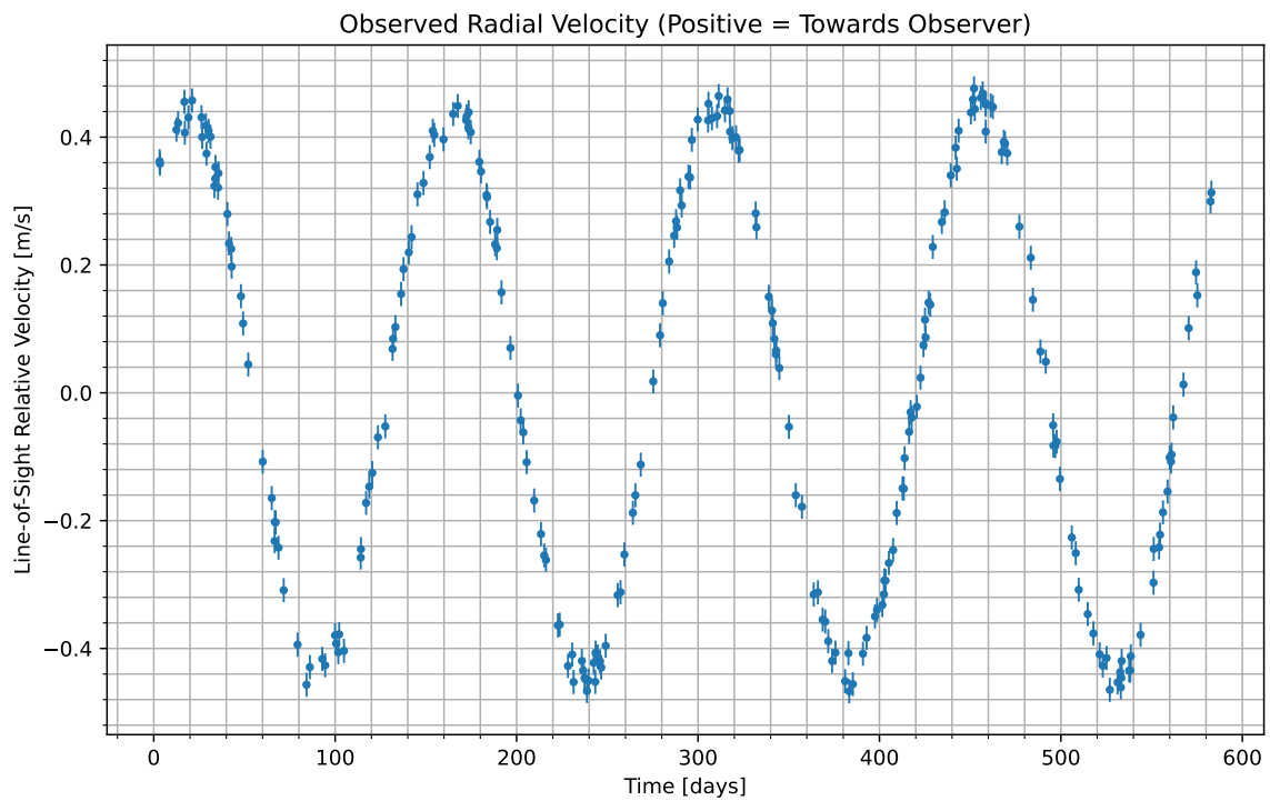
Figure 1: We have isolated the radial velocity of the host star due to the candidate planet. Data begins at UTC 2074-10-18/19:30. Positive values indicate the velocity at which the star is moving towards us; negative indicate the velocity at which it is moving away.
