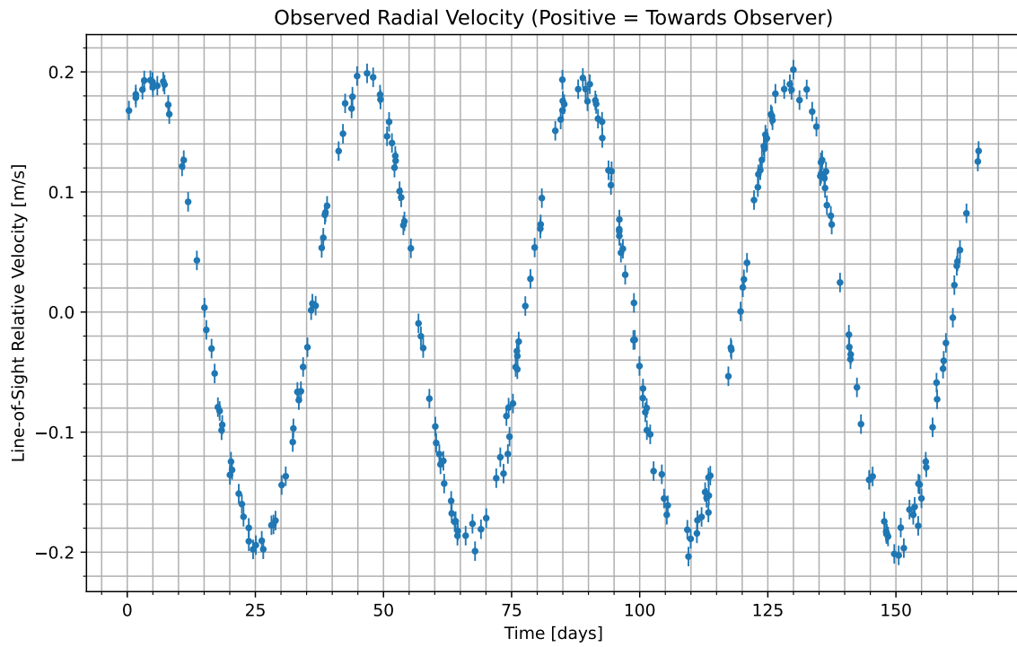
Figure 1: We have isolated the radial velocity of the host star due to the candidate planet. Data begins at UTC 2084-06-25/10:28. Positive values indicate the velocity at which the star is moving towards us; negative indicate the velocity at which it is moving away.
