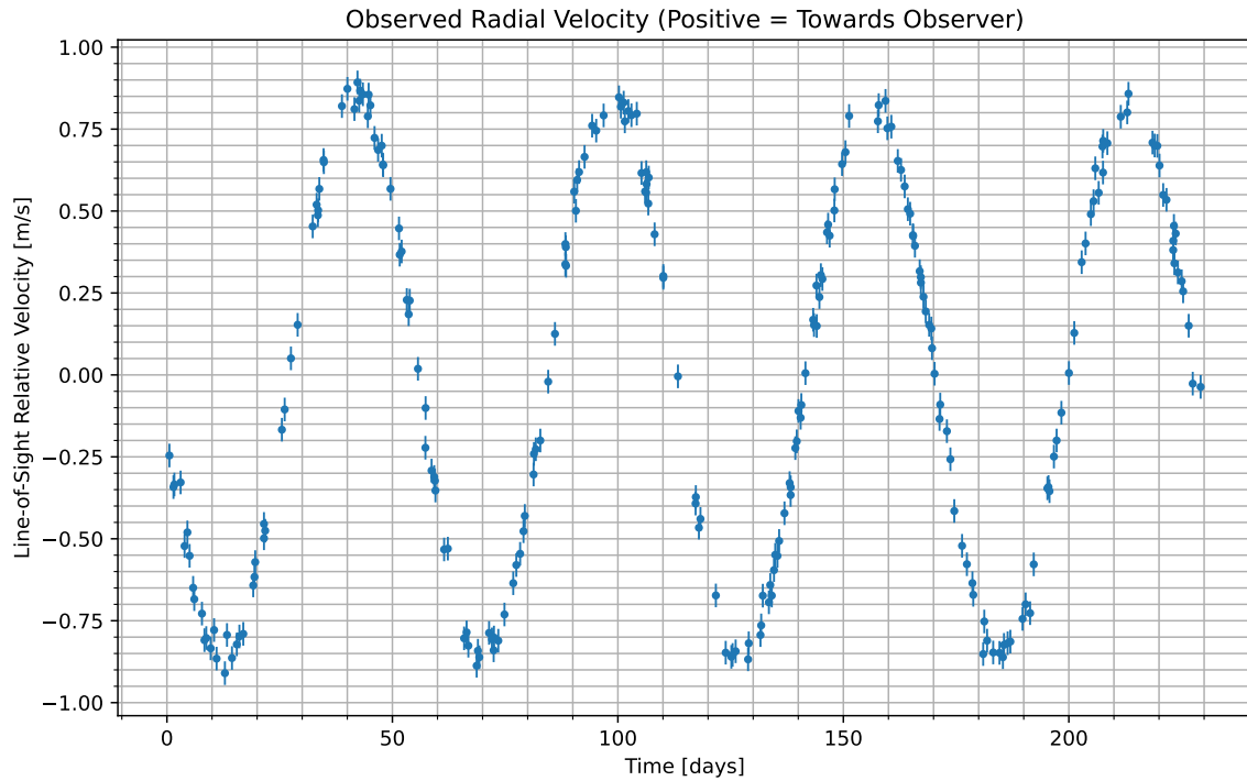
Figure 1: We have isolated the radial velocity of the host star due to the candidate planet. Data begins at UTC 2087-03-25/08:29. Positive values indicate the velocity at which the star is moving towards us; negative indicate the velocity at which it is moving away.
