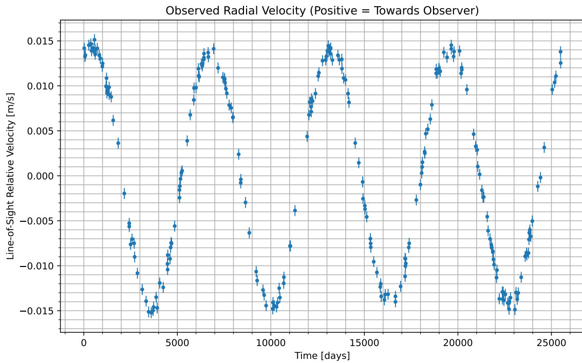
Figure 1: We have isolated the radial velocity of the host star due to the candidate planet. Data begins at UTC 2007-04-01/23:00. Positive values indicate the velocity at which the star is moving towards us; negative indicate the velocity at which it is moving away.
