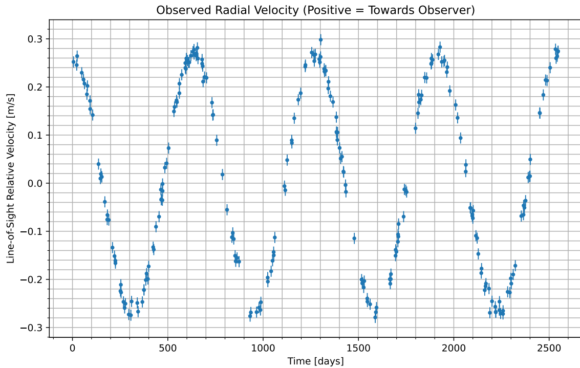
Figure 1: We have isolated the radial velocity of the host star due to the candidate planet. Data begins at UTC 2087-08-07/08:30. Positive values indicate the velocity at which the star is moving towards us; negative indicate the velocity at which it is moving away.
