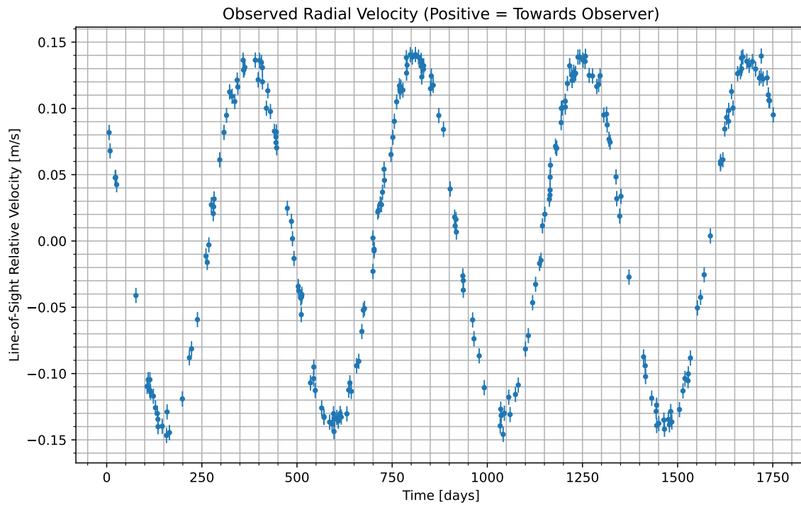
Figure 1: We have isolated the radial velocity of the host star due to the candidate planet. Data begins at UTC 2079-03-20/21:27. Positive values indicate the velocity at which the star is moving towards us; negative indicate the velocity at which it is moving away.
