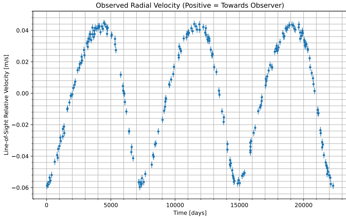
Figure 1: We have isolated the radial velocity of the host star due to the candidate planet. Data begins at UTC 2033-08-23/00:46. Positive values indicate the velocity at which the star is moving towards us; negative indicate the velocity at which it is moving away.
