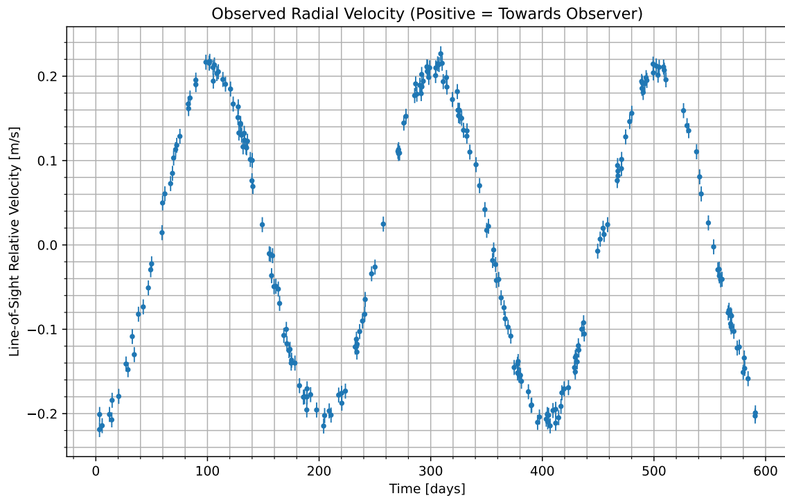
Figure 1: We have isolated the radial velocity of the host star due to the candidate planet. Data begins at UTC 2089-08-31/12:12. Positive values indicate the velocity at which the star is moving towards us; negative indicate the velocity at which it is moving away.
