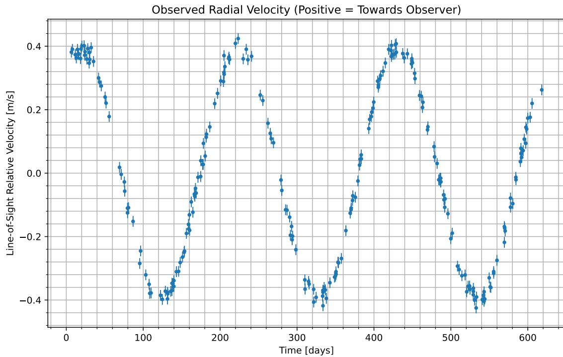
Figure 1: We have isolated the radial velocity of the host star due to the candidate planet. Data begins at UTC 2085-06-22/05:28. Positive values indicate the velocity at which the star is moving towards us; negative indicate the velocity at which it is moving away.
