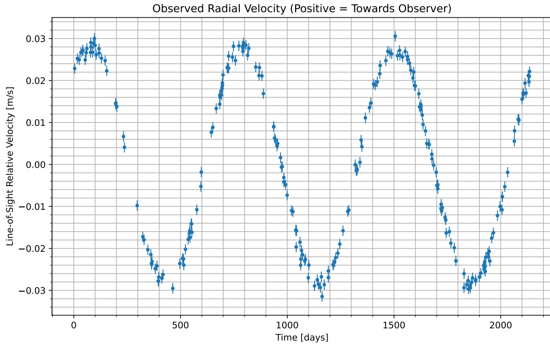
Figure 1: We have isolated the radial velocity of the host star due to the candidate planet. Data begins at UTC 2094-06-18/19:48. Positive values indicate the velocity at which the star is moving towards us; negative indicate the velocity at which it is moving away.
