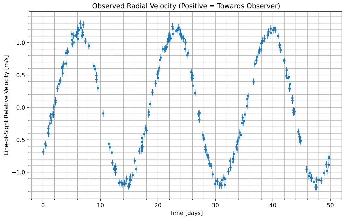
Figure 1: We have isolated the radial velocity of the host star due to the candidate planet. Data begins at UTC 2079-01-27/09:20. Positive values indicate the velocity at which the star is moving towards us; negative indicate the velocity at which it is moving away.
