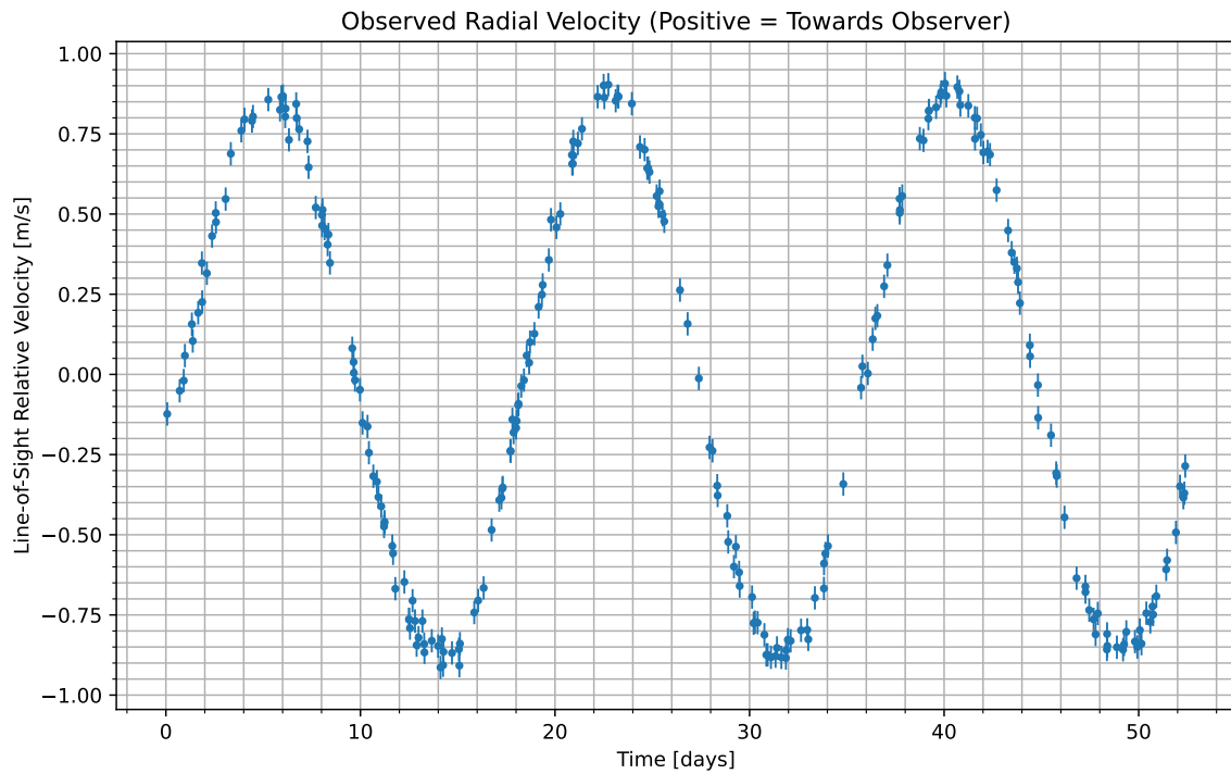
Figure 1: We have isolated the radial velocity of the host star due to the candidate planet. Data begins at UTC 2074-03-19/17:55. Positive values indicate the velocity at which the star is moving towards us; negative indicate the velocity at which it is moving away.
