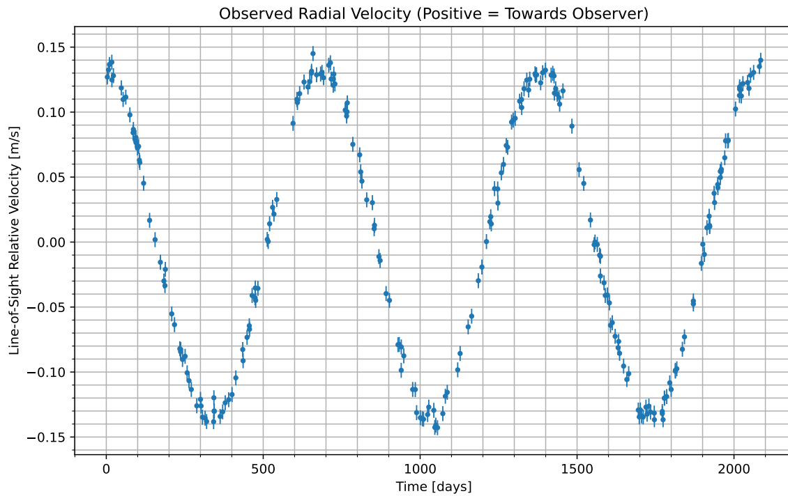
Figure 1: We have isolated the radial velocity of the host star due to the candidate planet. Data begins at UTC 2074-02-24/00:46. Positive values indicate the velocity at which the star is moving towards us; negative indicate the velocity at which it is moving away.
