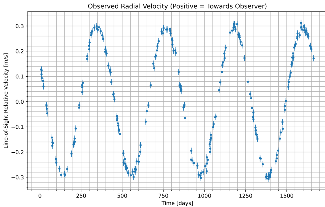
Figure 1: We have isolated the radial velocity of the host star due to the candidate planet. Data begins at UTC 2067-07-21/07:29. Positive values indicate the velocity at which the star is moving towards us; negative indicate the velocity at which it is moving away.
