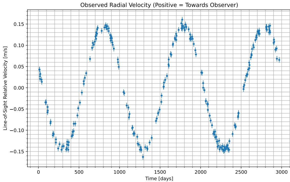
Figure 1: We have isolated the radial velocity of the host star due to the candidate planet. Data begins at UTC 2062-04-09/13:01. Positive values indicate the velocity at which the star is moving towards us; negative indicate the velocity at which it is moving away.
