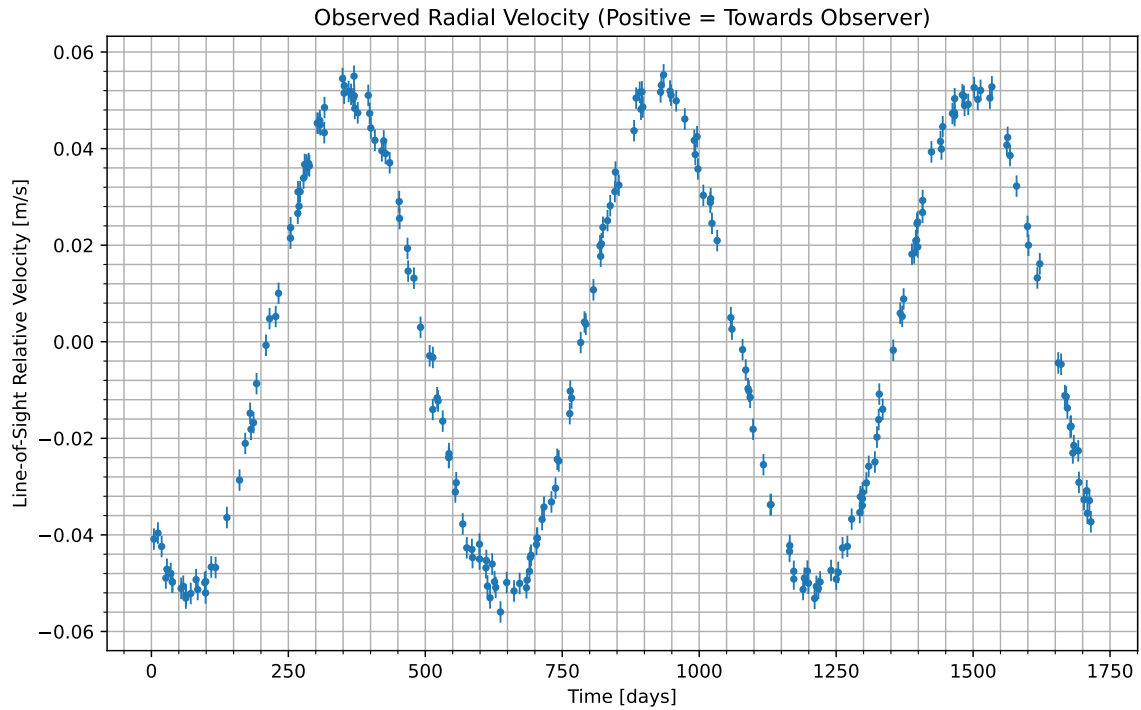
Figure 1: We have isolated the radial velocity of the host star due to the candidate planet. Data begins at UTC 2088-06-19/16:48. Positive values indicate the velocity at which the star is moving towards us; negative indicate the velocity at which it is moving away.
