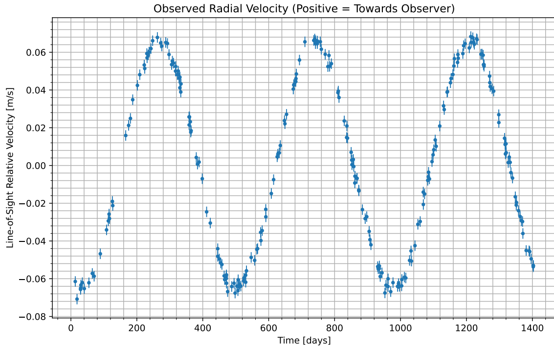
Figure 1: We have isolated the radial velocity of the host star due to the candidate planet. Data begins at UTC 2074-09-04/02:04. Positive values indicate the velocity at which the star is moving towards us; negative indicate the velocity at which it is moving away.
