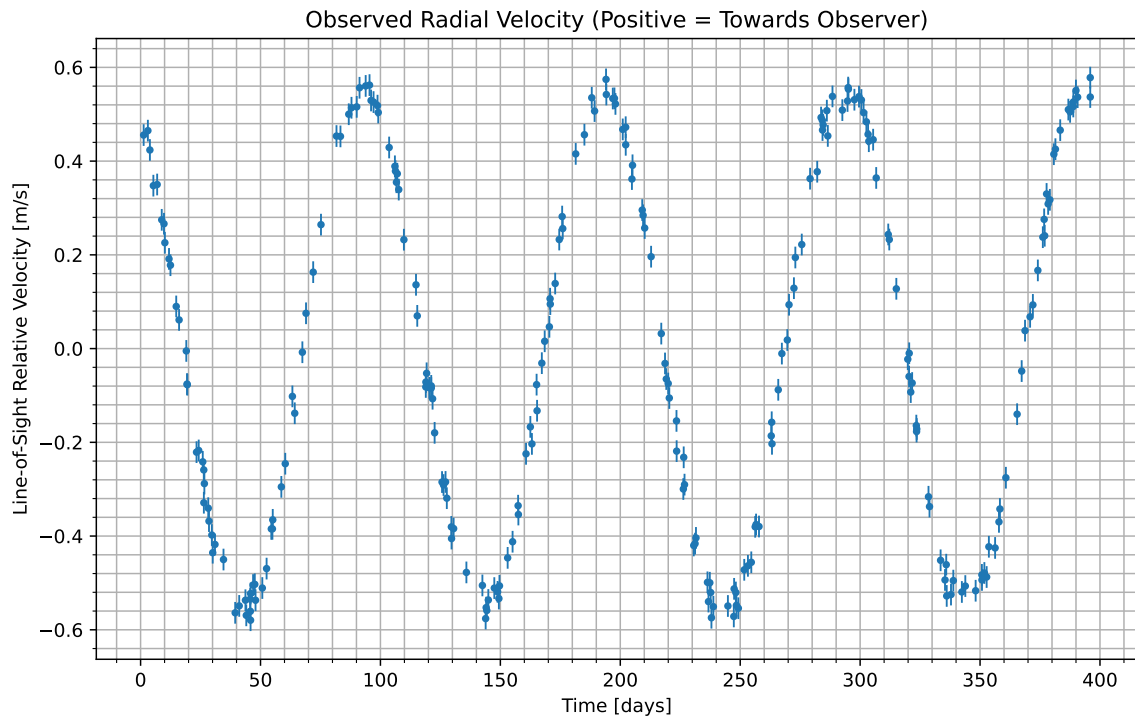
Figure 1: We have isolated the radial velocity of the host star due to the candidate planet. Data begins at UTC 2091-07-11/07:57. Positive values indicate the velocity at which the star is moving towards us; negative indicate the velocity at which it is moving away.
