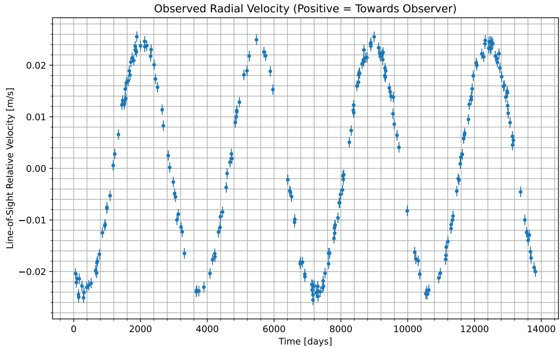
Figure 1: We have isolated the radial velocity of the host star due to the candidate planet. Data begins at UTC 2043-05-01/03:42. Positive values indicate the velocity at which the star is moving towards us; negative indicate the velocity at which it is moving away.
