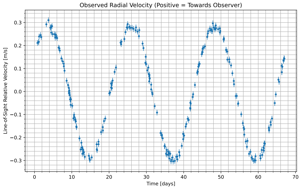
Figure 1: We have isolated the radial velocity of the host star due to the candidate planet. Data begins at UTC 2079-06-19/07:28. Positive values indicate the velocity at which the star is moving towards us; negative indicate the velocity at which it is moving away.
