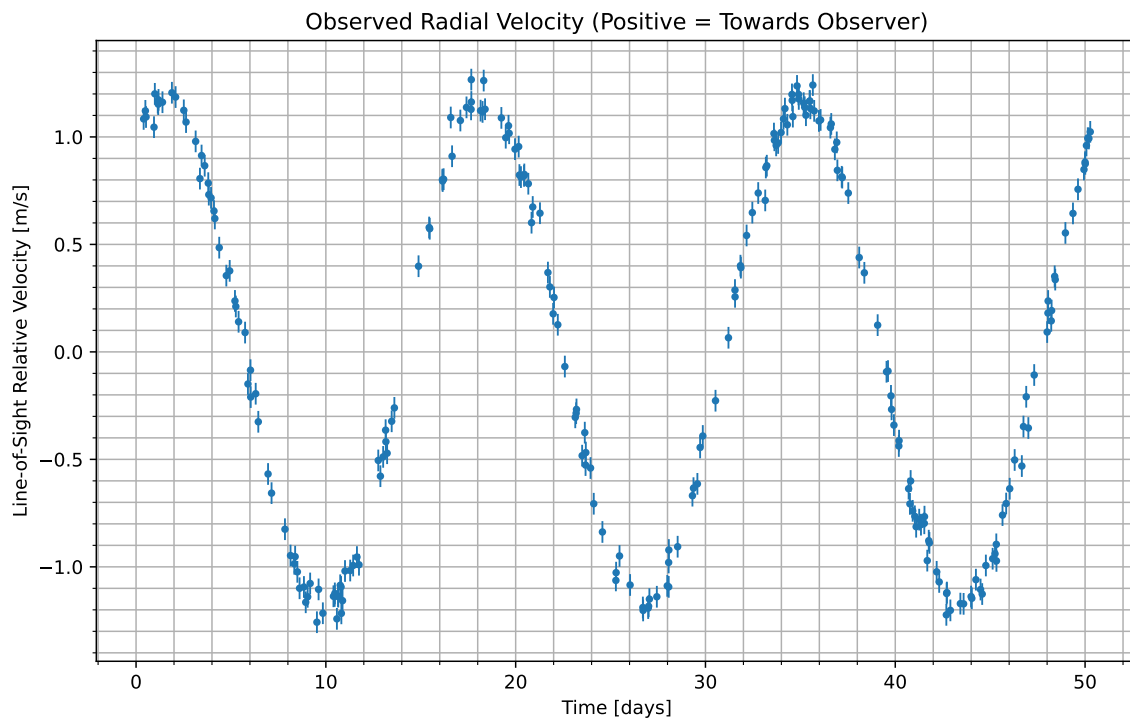
Figure 1: We have isolated the radial velocity of the host star due to the candidate planet. Data begins at UTC 2094-04-06/19:03. Positive values indicate the velocity at which the star is moving towards us; negative indicate the velocity at which it is moving away.
