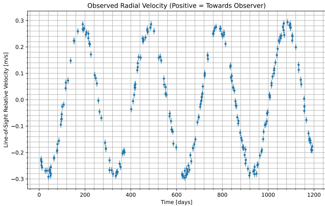
Figure 1: We have isolated the radial velocity of the host star due to the candidate planet. Data begins at UTC 2069-02-17/10:27. Positive values indicate the velocity at which the star is moving towards us; negative indicate the velocity at which it is moving away.
