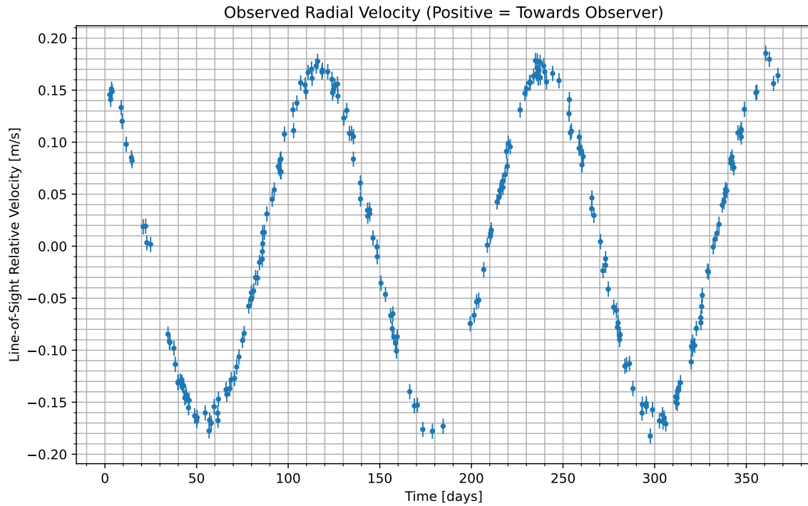
Figure 1: We have isolated the radial velocity of the host star due to the candidate planet. Data begins at UTC 2095-10-06/23:43. Positive values indicate the velocity at which the star is moving towards us; negative indicate the velocity at which it is moving away.
