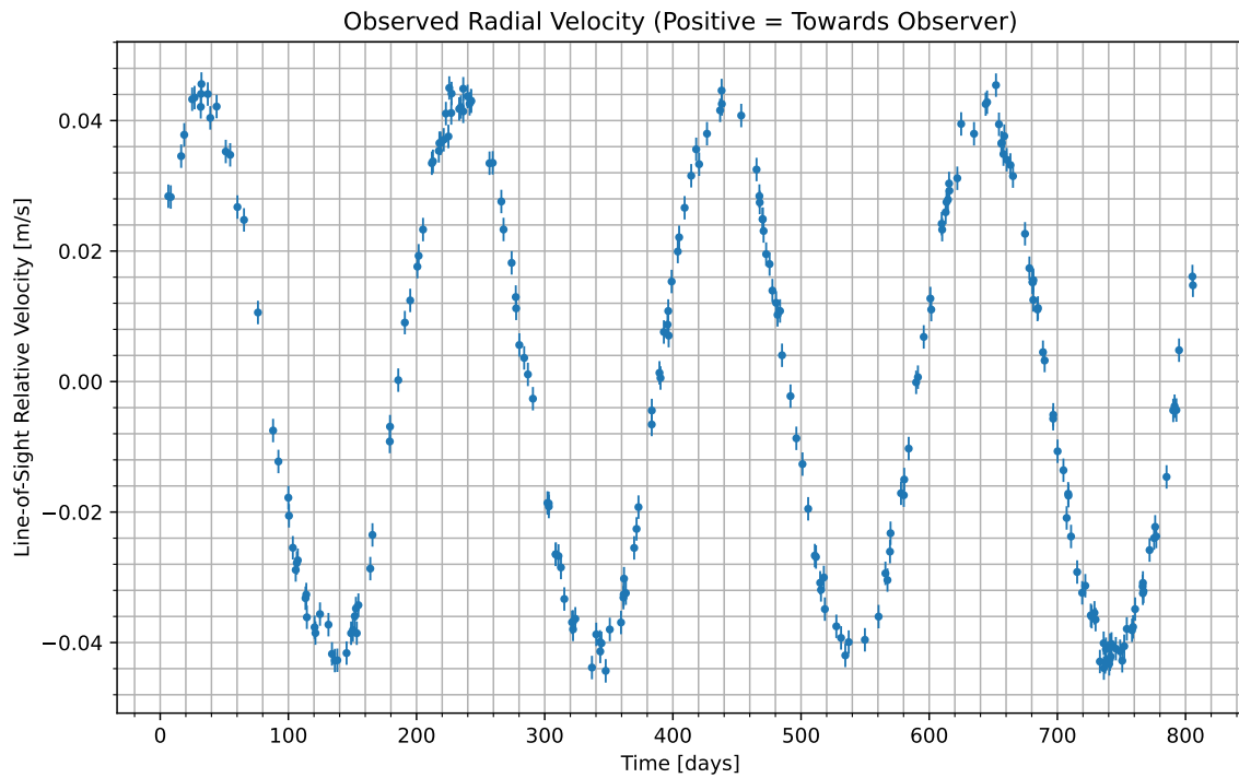
Figure 1: We have isolated the radial velocity of the host star due to the candidate planet. Data begins at UTC 2082-06-12/19:14. Positive values indicate the velocity at which the star is moving towards us; negative indicate the velocity at which it is moving away.
