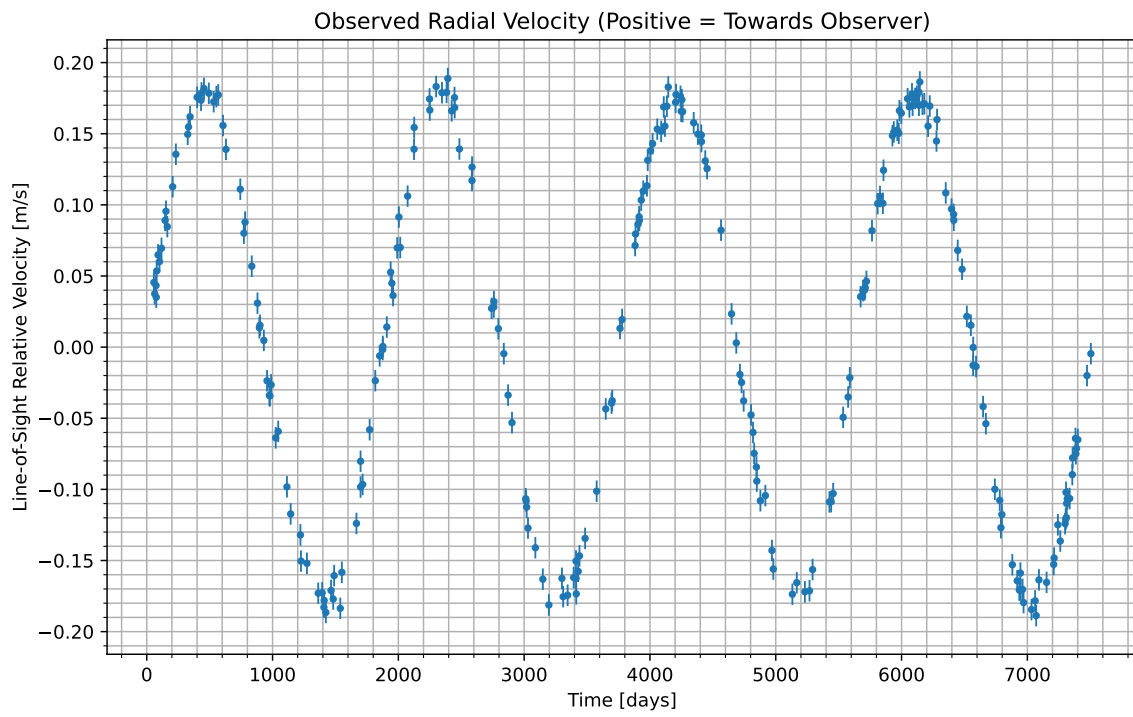
Figure 1: We have isolated the radial velocity of the host star due to the candidate planet. Data begins at UTC 2059-04-26/01:25. Positive values indicate the velocity at which the star is moving towards us; negative indicate the velocity at which it is moving away.
