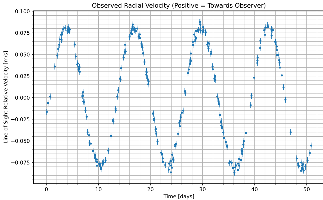
Figure 1: We have isolated the radial velocity of the host star due to the candidate planet. Data begins at UTC 2081-09-04/17:41. Positive values indicate the velocity at which the star is moving towards us; negative indicate the velocity at which it is moving away.
