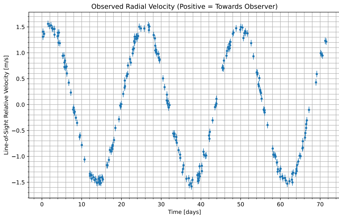
Figure 1: We have isolated the radial velocity of the host star due to the candidate planet. Data begins at UTC 2087-02-15/19:58. Positive values indicate the velocity at which the star is moving towards us; negative indicate the velocity at which it is moving away.
