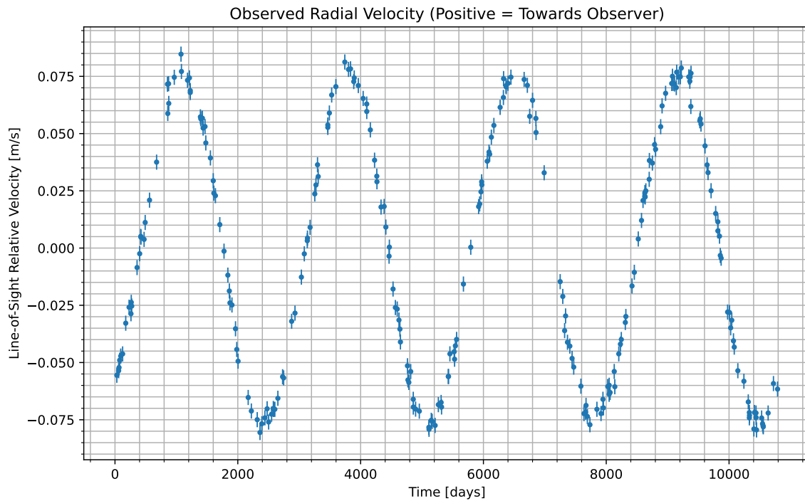
Figure 1: We have isolated the radial velocity of the host star due to the candidate planet. Data begins at UTC 2054-06-12/15:08. Positive values indicate the velocity at which the star is moving towards us; negative indicate the velocity at which it is moving away.
