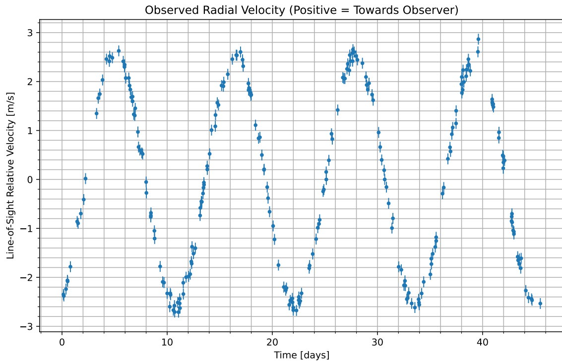
Figure 1: We have isolated the radial velocity of the host star due to the candidate planet. Data begins at UTC 2074-06-23/17:47. Positive values indicate the velocity at which the star is moving towards us; negative indicate the velocity at which it is moving away.
