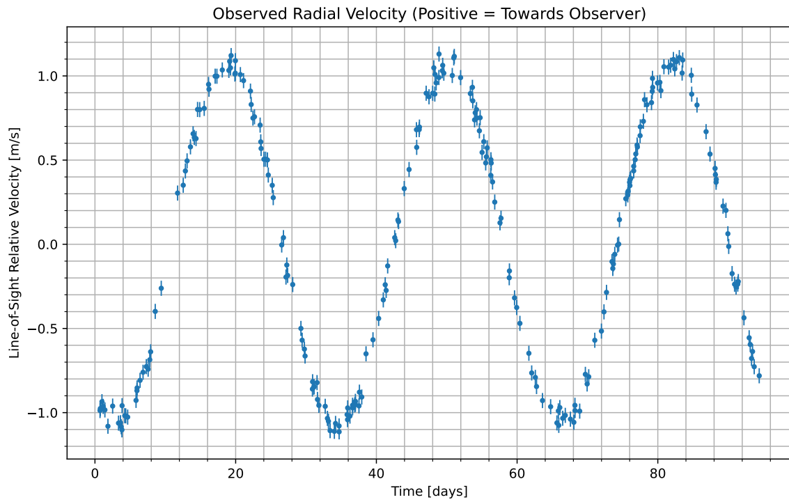
Figure 1: We have isolated the radial velocity of the host star due to the candidate planet. Data begins at UTC 2076-09-10/15:37. Positive values indicate the velocity at which the star is moving towards us; negative indicate the velocity at which it is moving away.
