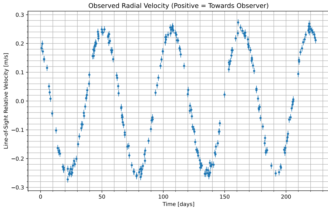
Figure 1: We have isolated the radial velocity of the host star due to the candidate planet. Data begins at UTC 2094-01-12/19:50. Positive values indicate the velocity at which the star is moving towards us; negative indicate the velocity at which it is moving away.
