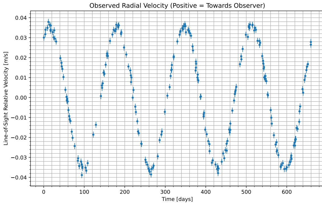
Figure 1: We have isolated the radial velocity of the host star due to the candidate planet. Data begins at UTC 2072-06-02/14:25. Positive values indicate the velocity at which the star is moving towards us; negative indicate the velocity at which it is moving away.
