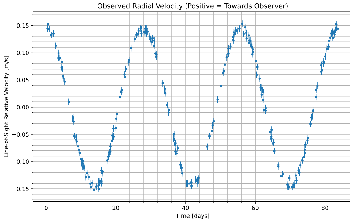
Figure 1: We have isolated the radial velocity of the host star due to the candidate planet. Data begins at UTC 2083-04-11/17:52. Positive values indicate the velocity at which the star is moving towards us; negative indicate the velocity at which it is moving away.
