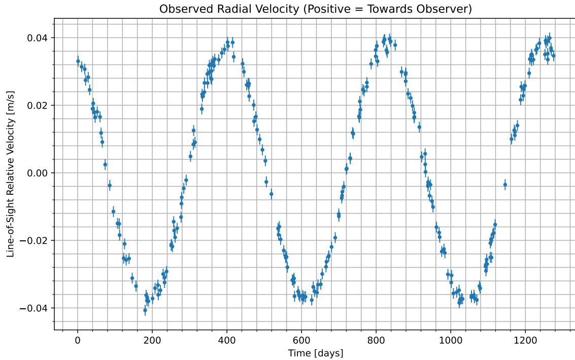
Figure 1: We have isolated the radial velocity of the host star due to the candidate planet. Data begins at UTC 2086-05-02/06:38. Positive values indicate the velocity at which the star is moving towards us; negative indicate the velocity at which it is moving away.
