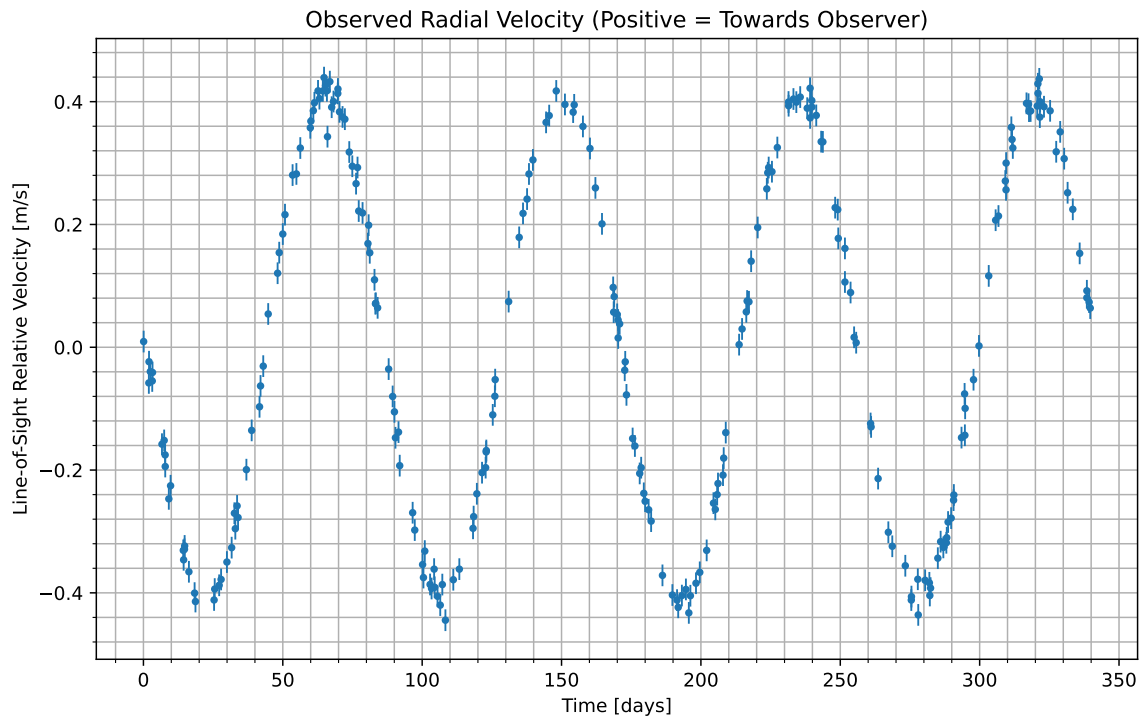
Figure 1: We have isolated the radial velocity of the host star due to the candidate planet. Data begins at UTC 2070-11-10/17:12. Positive values indicate the velocity at which the star is moving towards us; negative indicate the velocity at which it is moving away.
