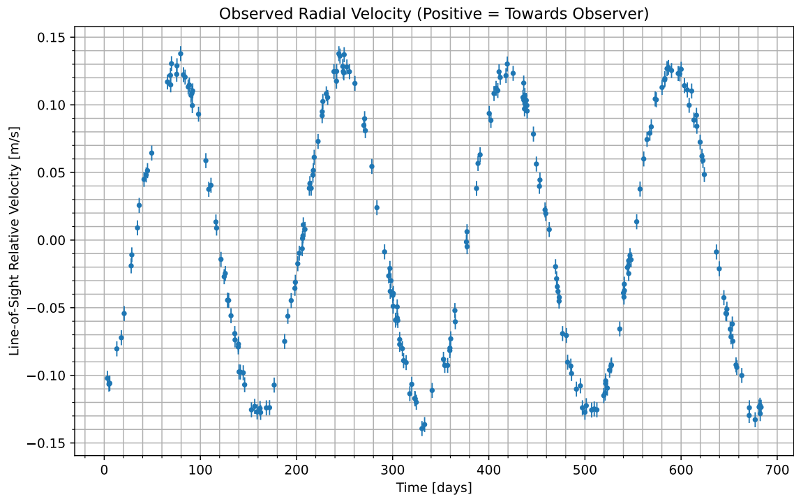
Figure 1: We have isolated the radial velocity of the host star due to the candidate planet. Data begins at UTC 2072-11-28/05:13. Positive values indicate the velocity at which the star is moving towards us; negative indicate the velocity at which it is moving away.
