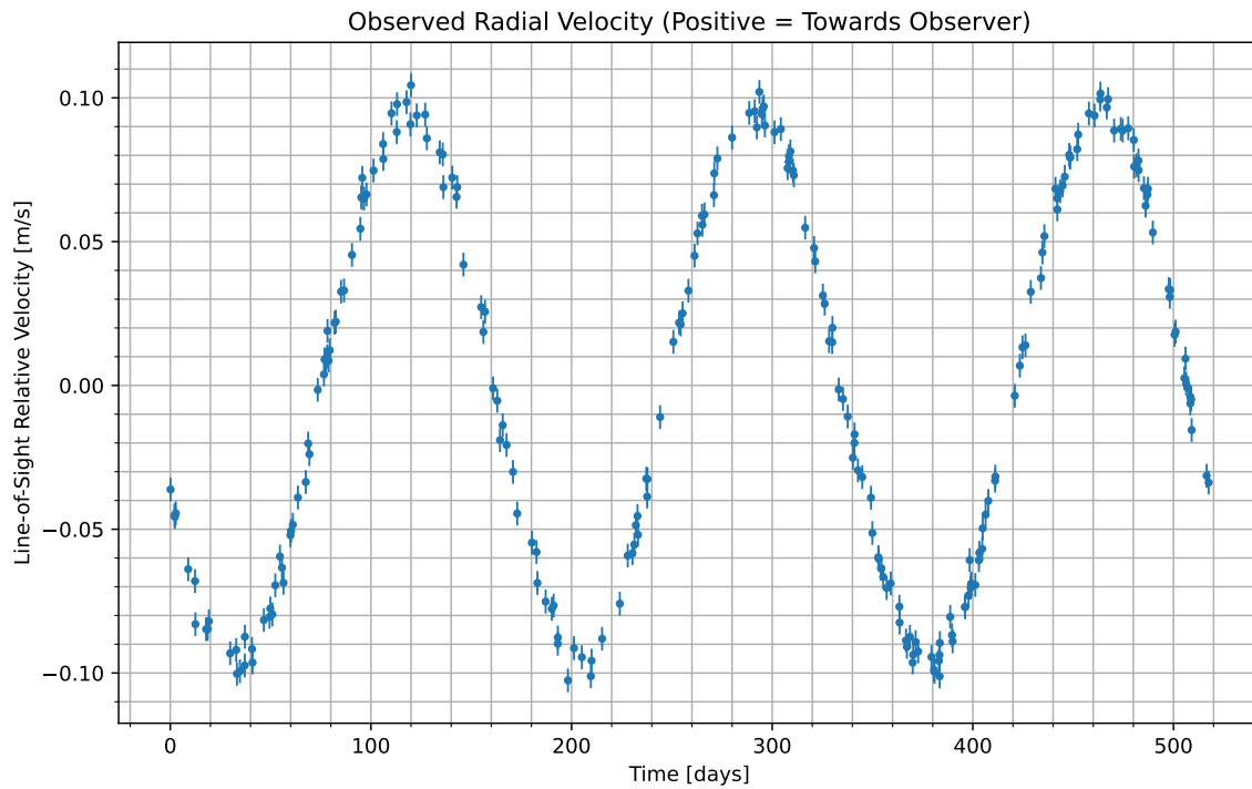
Figure 1: We have isolated the radial velocity of the host star due to the candidate planet. Data begins at UTC 2089-05-19/04:19. Positive values indicate the velocity at which the star is moving towards us; negative indicate the velocity at which it is moving away.
