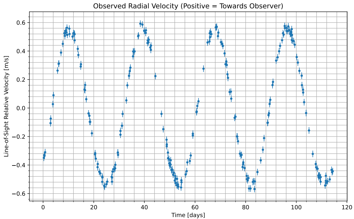
Figure 1: We have isolated the radial velocity of the host star due to the candidate planet. Data begins at UTC 2076-01-22/12:30. Positive values indicate the velocity at which the star is moving towards us; negative indicate the velocity at which it is moving away.
