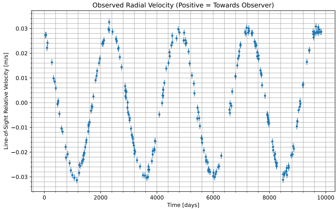
Figure 1: We have isolated the radial velocity of the host star due to the candidate planet. Data begins at UTC 2068-09-04/01:43. Positive values indicate the velocity at which the star is moving towards us; negative indicate the velocity at which it is moving away.
