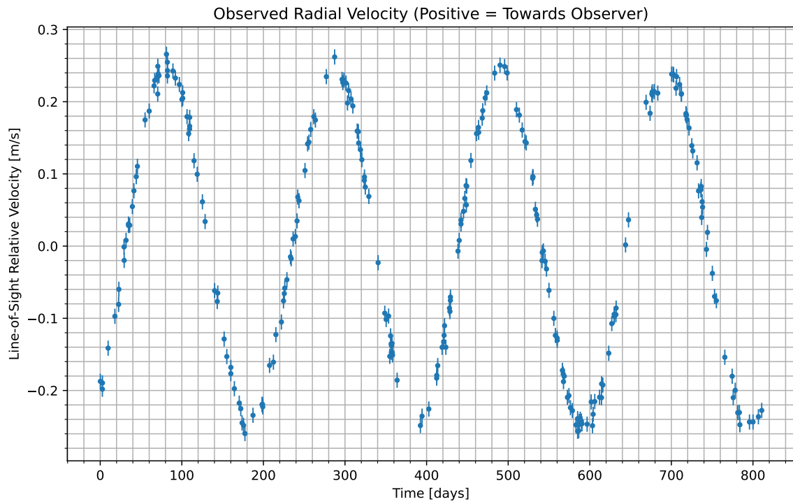
Figure 1: We have isolated the radial velocity of the host star due to the candidate planet. Data begins at UTC 2074-10-27/14:30. Positive values indicate the velocity at which the star is moving towards us; negative indicate the velocity at which it is moving away.
